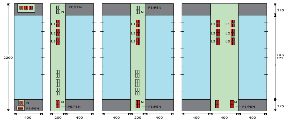
Busbar System 2
