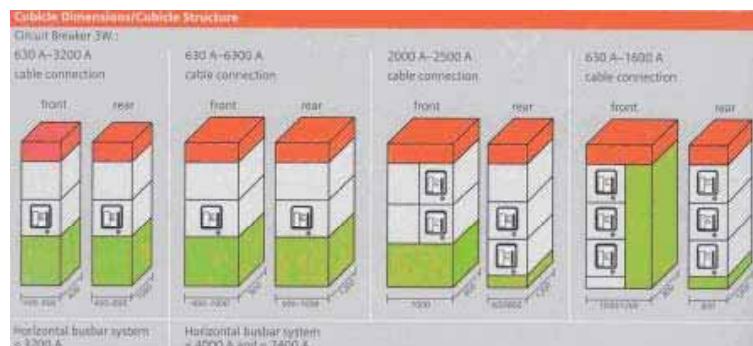
Circuit Breaker Cabinet 3
